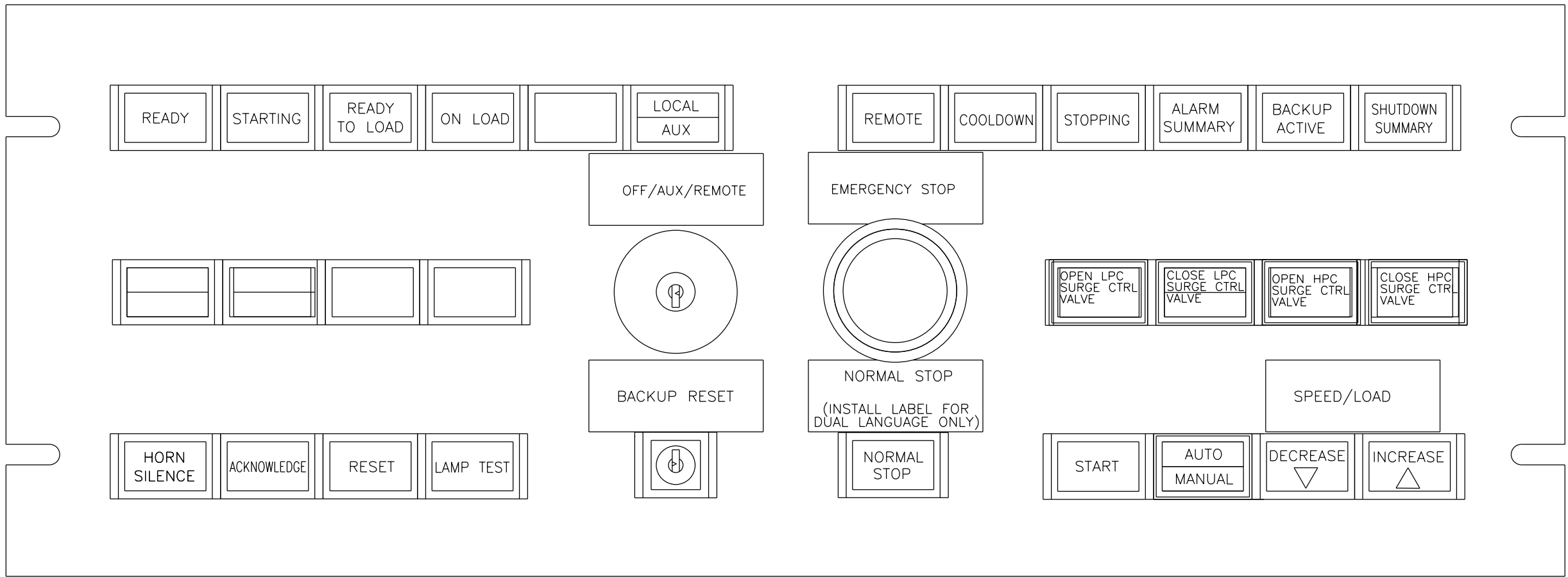
FRONT VIEW
