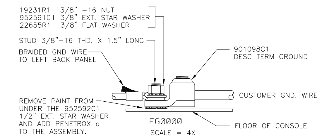
TYPICAL GROUND STUD ASSEMBLY
